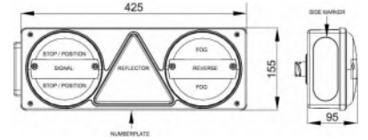
Without LED Side Lamp LED Yan Lambasız
