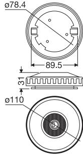
Cast Aluminium Chrome Plated Ø80 mm
